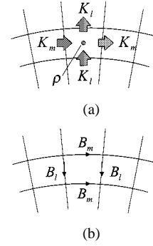
Fig. 3. (a) Allocation of surface charge and current density. (b) Allocation of associated magnetic field components.
